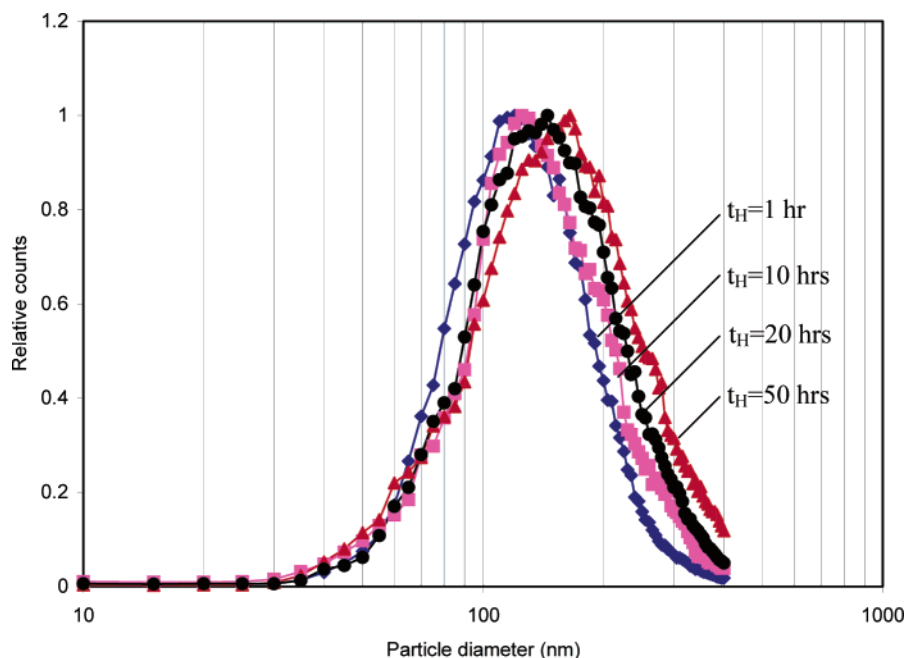
Figure 2. Particle size distribution for various aging times of the precursor solution (TEOS/EtOH/H 2 O/HCl/NaCl = 1:22:60:30:2).
