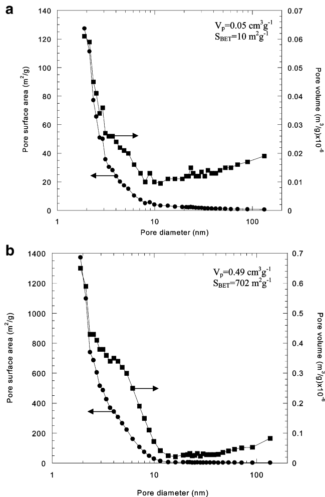
Figure 4. Pore surface area and volume distribution (a) before and (b) after salt removal ( t_H = 50 h, BJH adsorption curve).
