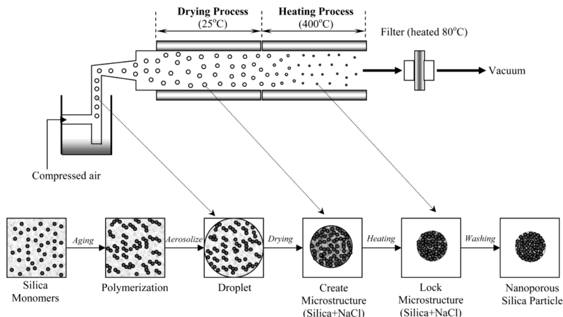
Figure 1. The schematic of the experimental setup and an illustration of the possible pathway of nanoporous silica particle formation.
