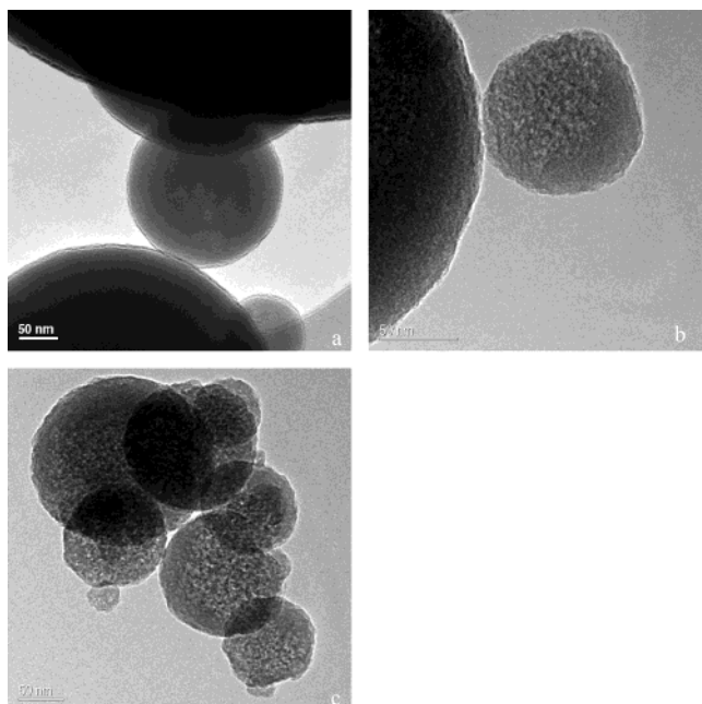
Figure 3. TEM images of silica particles: (a) TEOS/EtOH/H 2 O/HCl/NaCl = 1:22:60:30:0 ( t_H = 20 h), (b) TEOS/EtOH/H 2 O/HCl/NaCl = 1:22:60:30:2 ( t_H = 20 h), and (c) TEOS/EtOH/H 2 O/HCl/NaCl = 1:22:60:30:2 ( t_H = 50 h).
