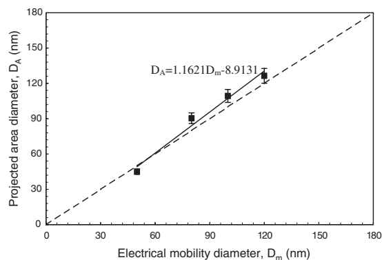
Figure 5. Comparison of the projected area diameter of nanotubes (from TEM) with the electrical mobility diameter (from electrophoretic separation). The dotted line is for D_A = D_m .
