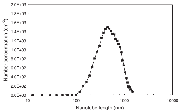
Figure 6. Length distribution of nanotubes classified by the electrostatic classifier.
