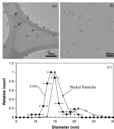
Figure 2. TEM images of (a) fully sintered Ni particles and (b) CNTs grown on the size-selected Ni particles, and the relative size distribution of Ni particles and CNTs measured by tandem electrostatic classifiers and TEM (digital image software), respectively.
