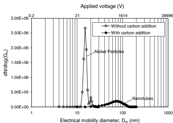
Figure 3. Number distribution of sintered size-selected nickel nanoparticles and nanotubes grown on the nickel nanoparticles as a function of electrical mobility diameter. (Experimental conditions: geometry of electrostatic classifier: r_1 = 0.937 cm (inner radius of electrode), r_2 = 1.961 cm (radius of housing), L = 44.369 cm (electrode length) and Q_{sh} = 10 lpm (sheath flow rate)).
