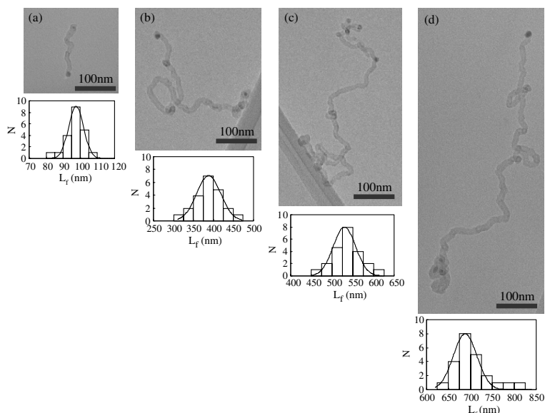
Figure 4. TEM images of uniform diameter nanotubes length-classified by gas phase electrophoresis at an equivalent electrical mobility diameter (applied voltage) of (a) D_m = 50 nm (465 V), (b) D_m = 80 nm (1089 V), (c) D_m = 100 nm (1607 V) and (d) D_m = 120 nm (2199 V) in the second electrostatic classifier.
