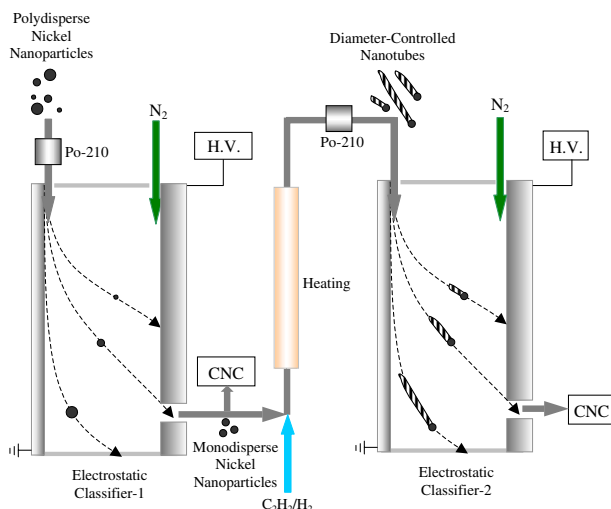
Figure 1. Schematic diagram of the length classification of nanotubes by gas phase electrophoresis using tandem mobility analysers. (H.V.: high voltage power supply, CNC: condensation nucleus counter).
